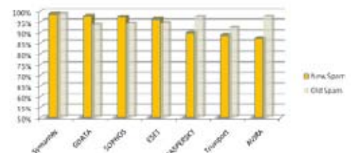
SPAM-Test Results
